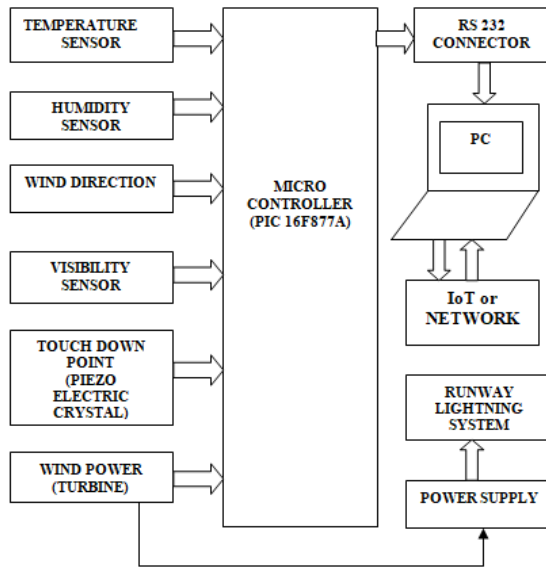
Figure 3: Block diagram
