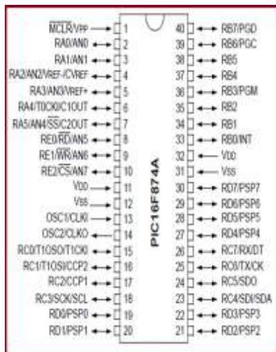
Figure 4: Pin configuration
