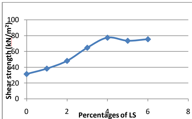
Fig 7 Variation of shear strength with the addition of lignosulfonate
